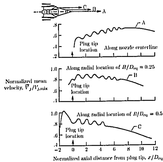
(a) Supersonic inner stream; NPR_i = 3.14 ; NPR_o = 3.33 ; T_{T,i} = 870^\circ R ; T_{T,o} = 1670^\circ R .
