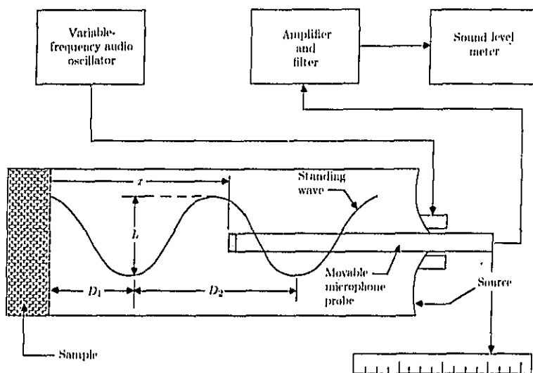
Figure 10. Normal-incidence impedance tube apparatus. (From ref. 7.)
