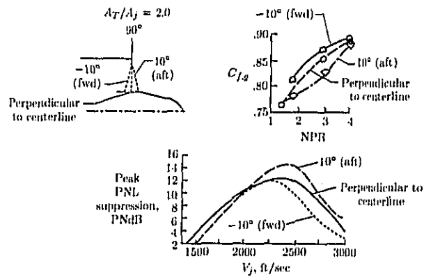
(e) Influence of element cant angle on acoustic and aerodynamic performance.
