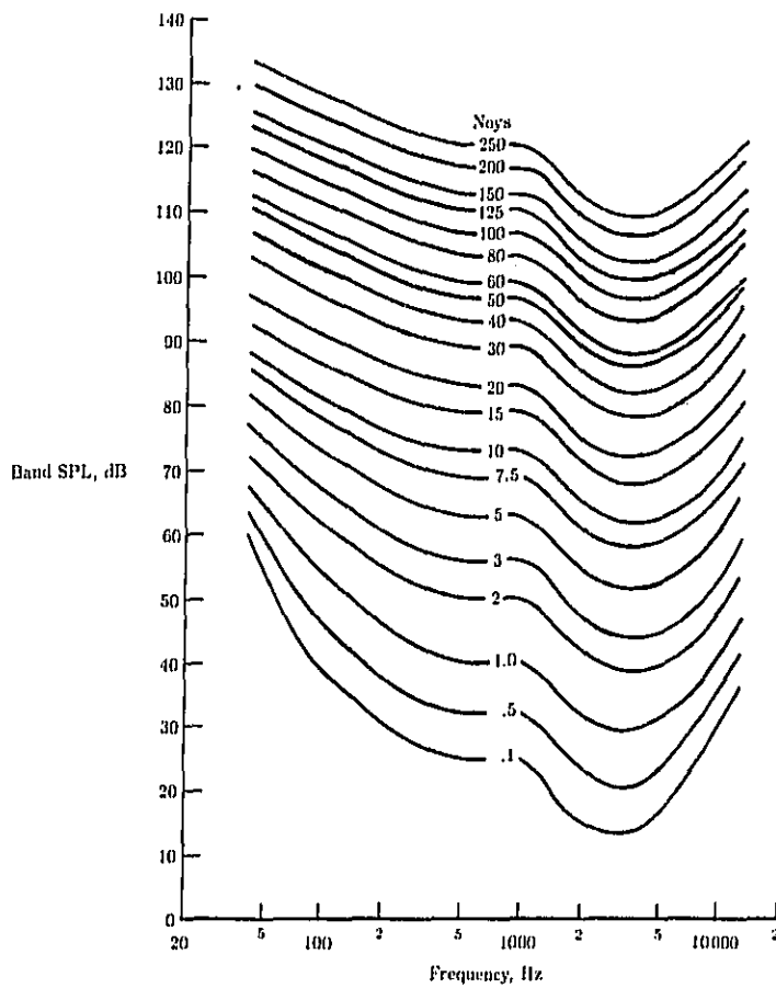
Figure 9. Equal-noisiness contours. (From ref. 14.)
