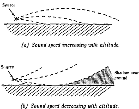
Figure 9. Schematic showing the bending of ray paths.
