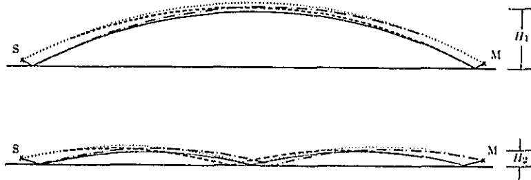
Figure 12. Schematic showing groups of ray paths in downward refraction that have approximately the same heights at zenith. (From ref. 25.)
