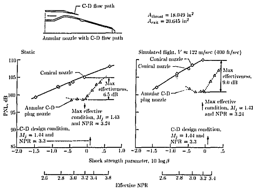
(a) Effectiveness of C-D flow path in shock noise reduction for annular plug nozzle in terms of PNL at \theta_i = 60^\circ . Data scaled to A_T = 0.903 \text{ m}^2 (1400 \text{in}^2 ) and 792-m (2400-ft) sideline.
