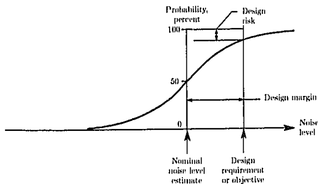
Figure 9. Design margin and risk.
