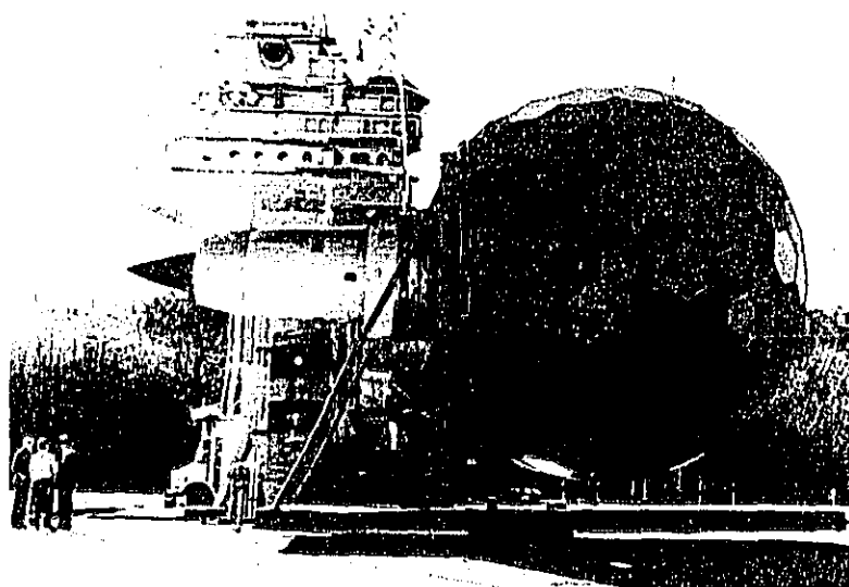
Figure 11. Fan flight noise simulation full-scale testing.
