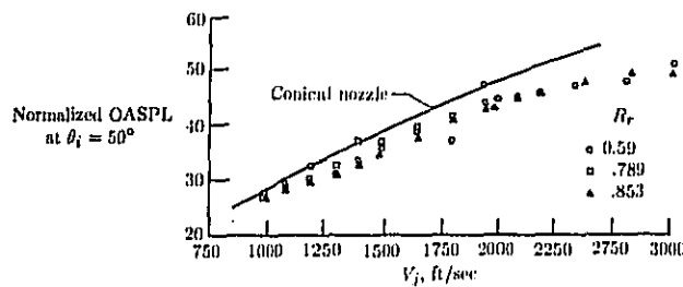
(b) OASPL at \theta_i = 50^\circ .
