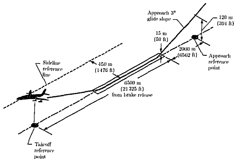
Figure 1. FAR Part 36 noise certification conditions.
