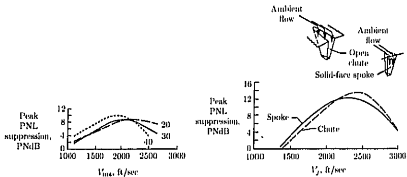
(c) Peak PNL suppression as function of suppressor element number; static; A_T/A_j = 1.75 ; R_r = 0.717 ; scaled to A_T = 338 \text{ in}^2 .
