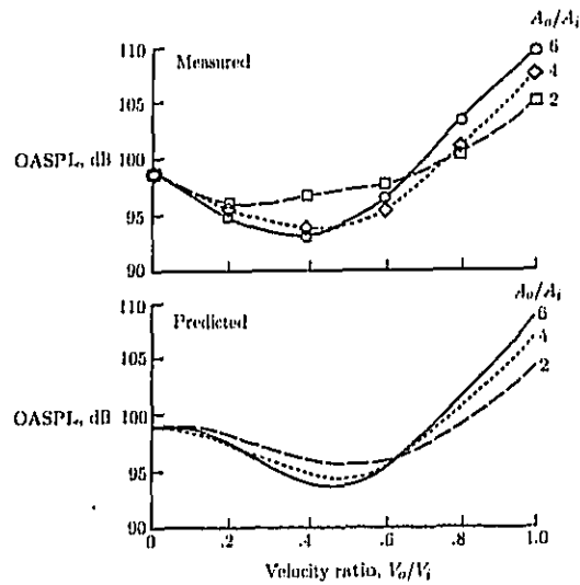
Figure 4. Influence of area ratio on conventional bypass jet OASPL. \theta = 90^\circ ; V_i = 305 m/sec; T_{i,i} = 700 K; T_{T,o} = 300 K. (From ref. 11.)
