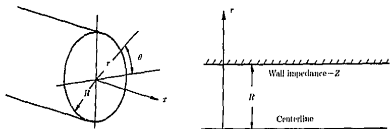
(a) Cylindrical coordinate system.
