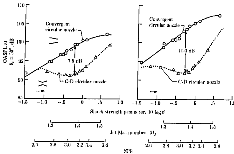
(a) Effectiveness of C-D flow path on circular nozzle in reduction of shock-cell noise. Data scaled to A_T = 1400 \text{ in}^2 and extrapolated to 2400-ft sideline; T_T = 1700^\circ \text{ R} .
