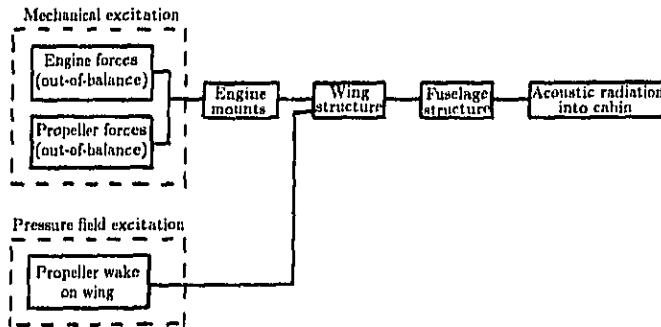
Figure 98. Main components of structure-borne sound transmission path for twin-engine airplane.
