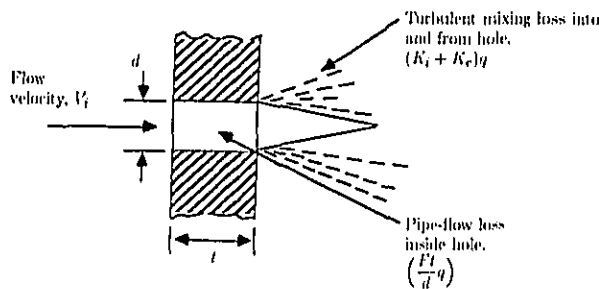
Figure 5. Flow mechanisms for dc flow resistance.
