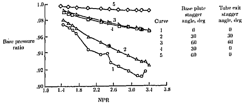
(b) Aerodynamic performance; A_T/A_j = 2.0 .
