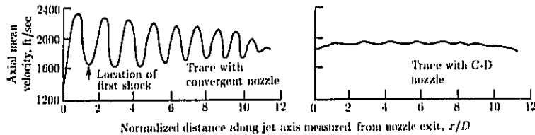
(b) Plume velocity data for conical and C-D nozzles. V = 400 ft/sec; T_T = 1720^\circ R ; NPR = 3.12 .
