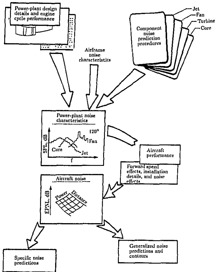
Figure 7. Elements necessary for noise prediction.
