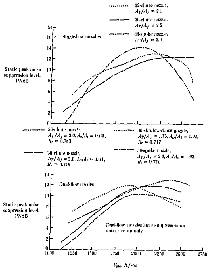
Figure 22. Typical static peak/PNL suppression characteristics of multi-element suppressors. 2400-ft sideline; standard day ( 59^\circ , 70 percent relative humidity); A_T = 338 \text{ in}^2 . (Based on ref. 20.)
