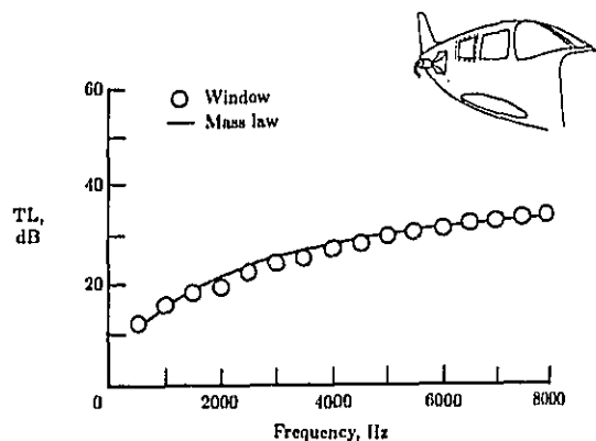
Figure 40. In-place measurement (ref. 129) of aircraft window noise transmission loss using acoustic intensity.
