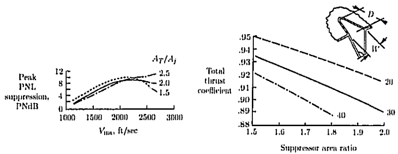
(a) Influence of 36-chute suppressor area ratio on peak PNL suppression; 2400-ft sideline; dual flow; scaled to A_T = 338 \text{ in}^2 .
