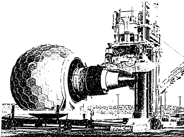
Figure 22. Full-scale engine test facility with turbulence control structure.
