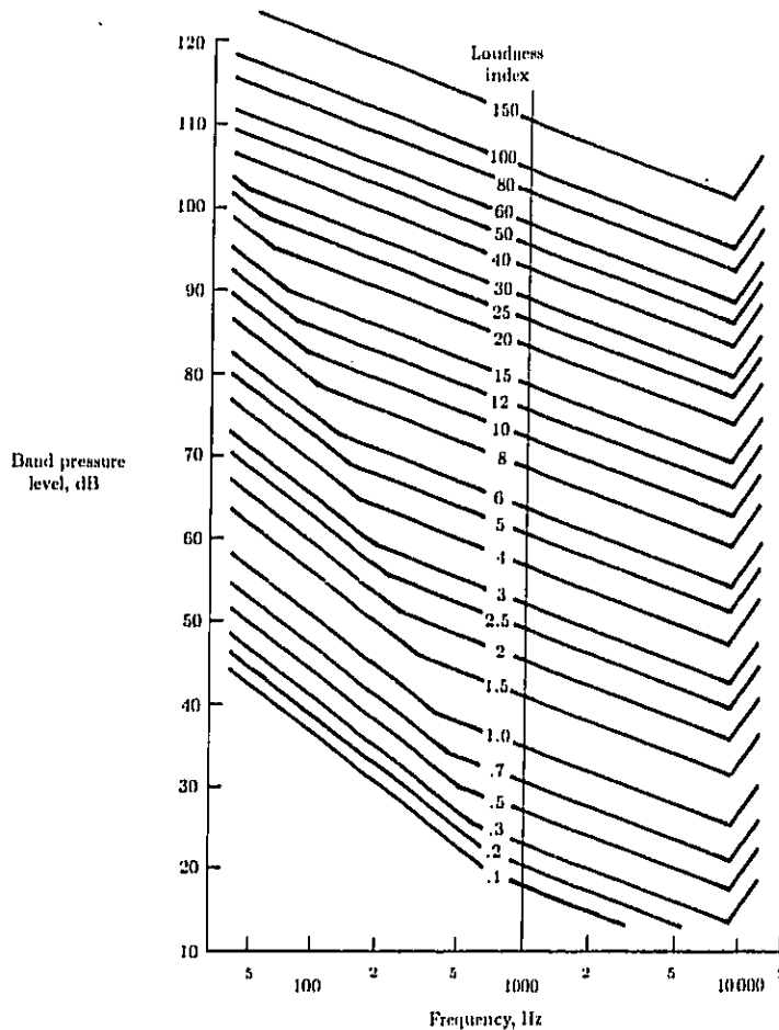
Figure 6. Frequency characteristics for the Mark VI loudness procedure. (From ref. 19.)
