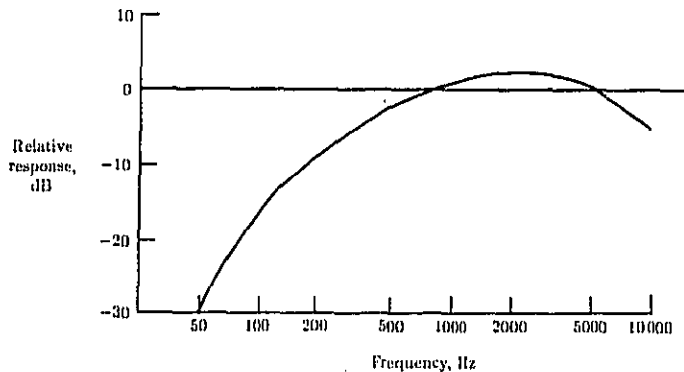
Figure 5. Relative response of the A-weighting filter.
