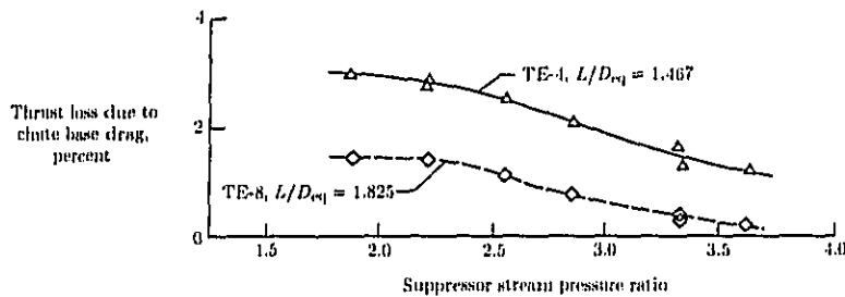
(b) Simulated flight, V = 400 ft/sec.
