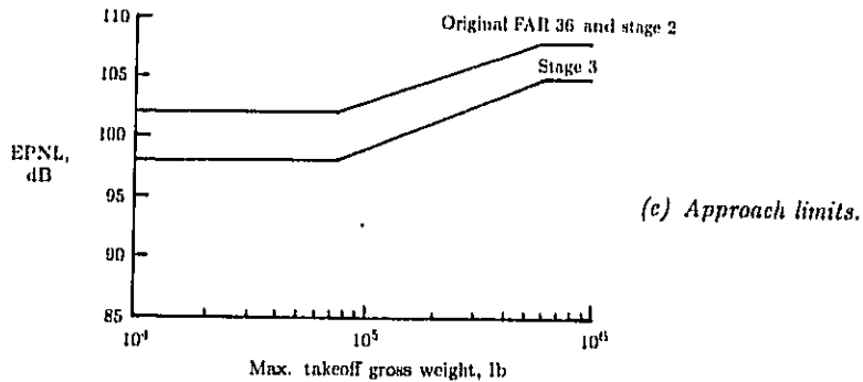
Figure 24. FAR 36 noise limits for transport aircraft.
