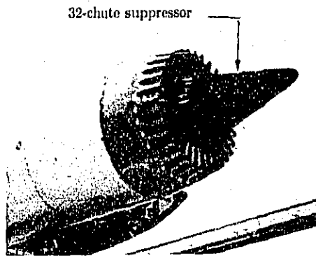
(a) Suppressor installed on J-79 engine.
