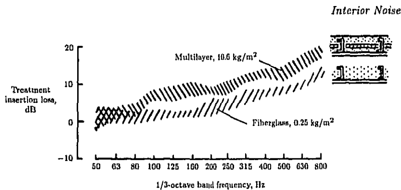
Figure 12. Insertion loss of add-on sidewall treatment for cabin noise control measured in flight of a light twin-engine propeller aircraft (ref. 32). Insertion loss equals SPL before treatment minus SPL after treatment.
