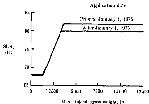
Figure 25. FAR 36 noise limits for small propeller-driven aircraft.
