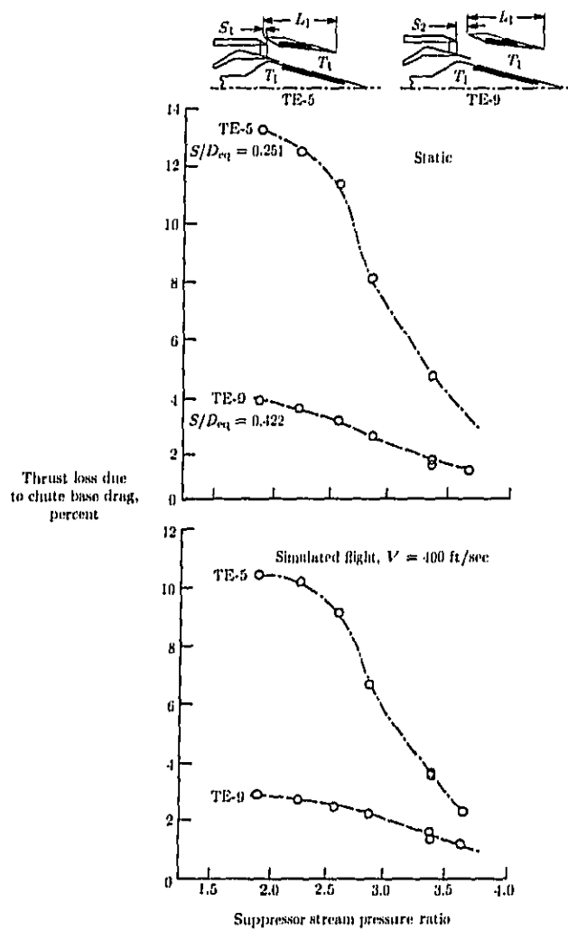
Figure 39. Influence of ejector spacing on base drag of 20-shallow-chute suppressor nozzle (dual flow). (Based on ref. 25.)
