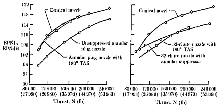
Figure 44. Integration study results of TAS implementation by bleeding. 305-m (1000-ft) level flyover at V = 122 m/sec (400 ft/sec). (From ref. 33.)
