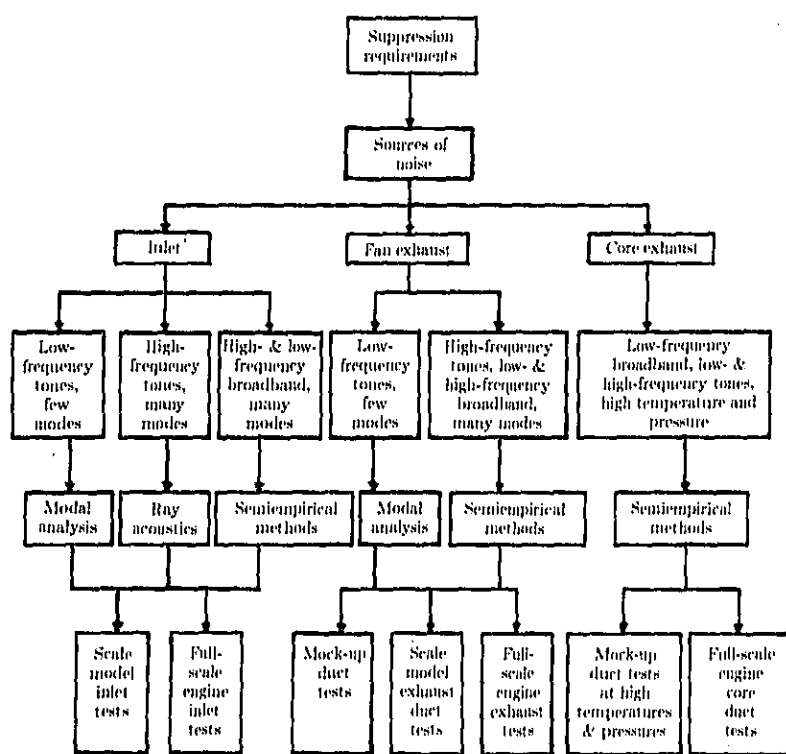
Figure 2. Schematic of engine treatment design approaches.
