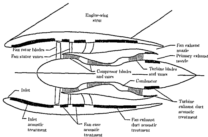
Figure 10. High-bypass-ratio engine and nacelle.
