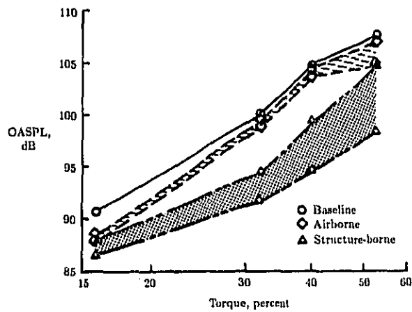
Figure 96. Airborne and structure-borne sound levels deduced from measurements in passenger compartment of a twin-engine, propeller-driven airplane. (From ref. 101.)
