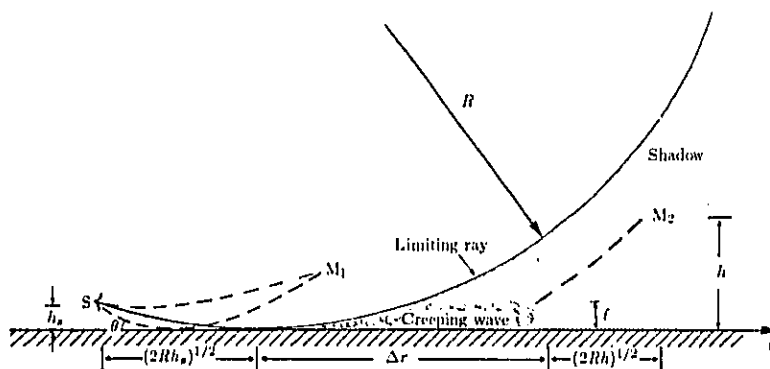
Figure 19. Schematic illustrating the main features of upward refraction. (From ref. 31.)
