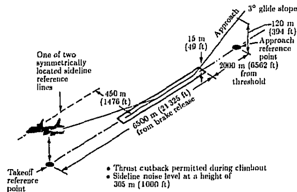
Figure 1. Noise certification measurement locations for new designs.
