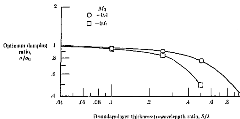
Figure 6. Effect of ratio of boundary-layer thickness to wavelength on ratio of maximum attenuation with boundary layer to maximum attenuation without boundary layer. m = 7 mode; \tau_1 = 10\pi .
