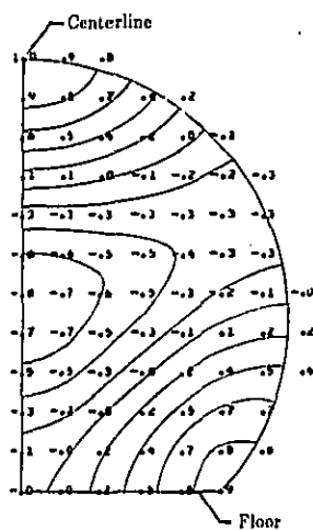
Figure 14. Acoustic mode shape of a cylindrical fuselage with an integral floor, calculated using finite difference method (ref. 48). Numbers are modal amplitudes.
