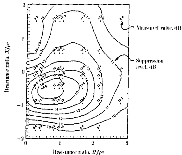
Figure 18. Example of isosuppression contours drawn in impedance plane.
