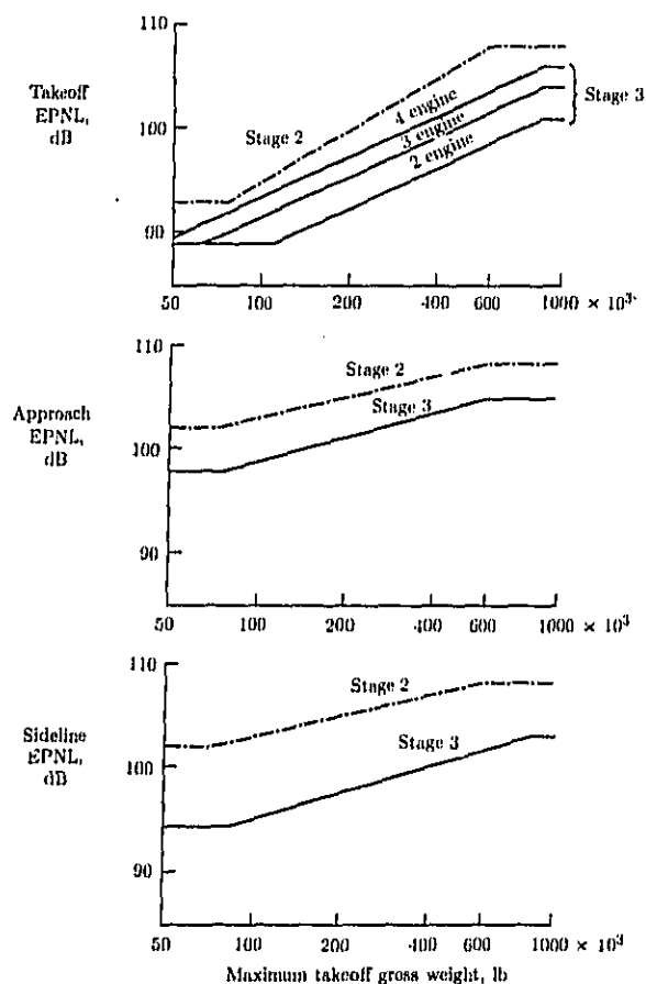
Figure 2. FAR Part 36 certification noise rules.
