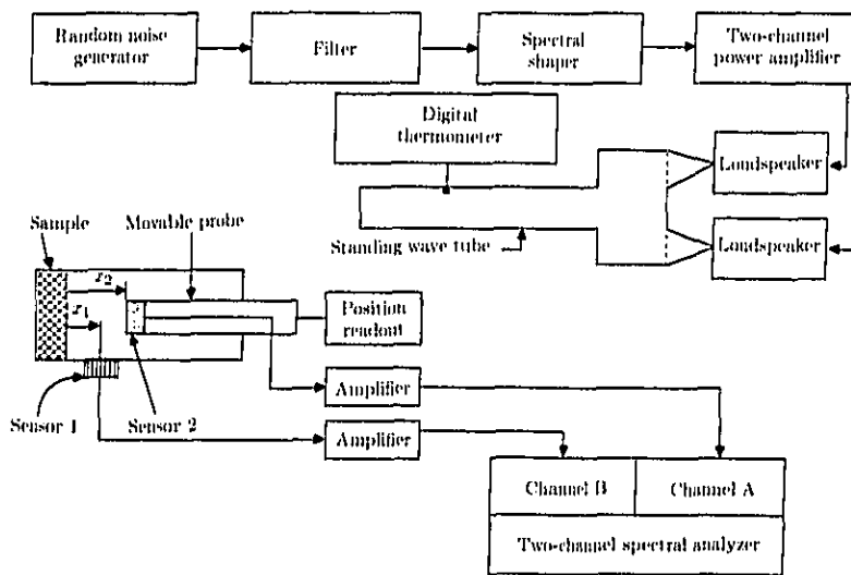
Figure 11. Dual-sensor method for normal-incidence impedance measurement.
