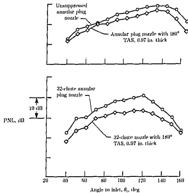
Figure 43. Influence of TAS on PNL directivity of unsuppressed annular plug and 32-chute suppressed nozzles at cutback cycle. A_T = 1400 \text{ in}^2 ; 1000-ft flyover distance; static operation. (Based on ref. 33.)
