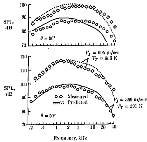
Figure 3. Conical nozzle predicted and measured SPL spectra. (From ref. 11.)
