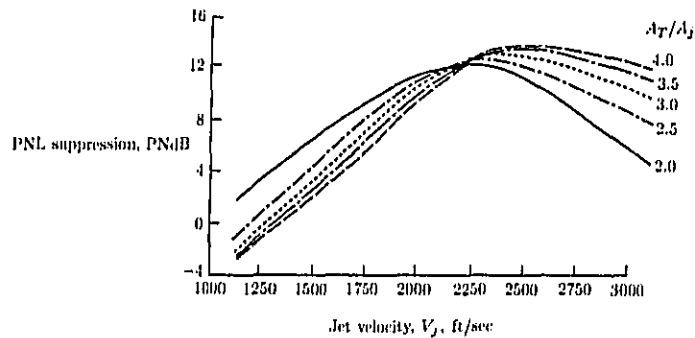
(a) PNL suppression; 1500-ft sideline; no shroud; based on data at A_T/A_j = 2.0, 2.3, 2.7, 3.1, \text{ and } 4.0 (2.0 and 4.0 repeated).
