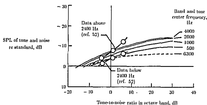
Figure 19. Effect of tone-to-noise ratio on noisiness. (From ref. 51.)
