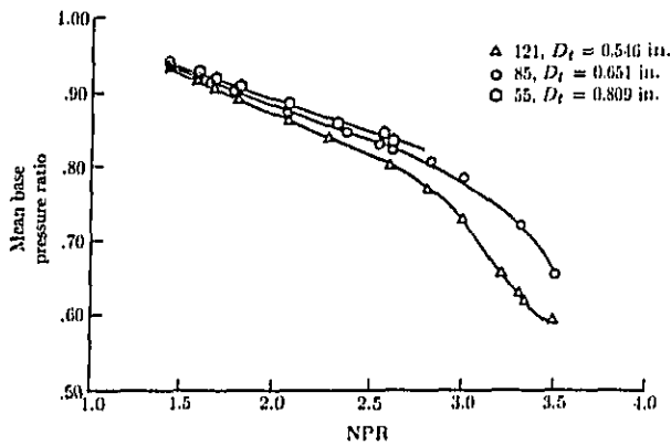
(b) Base pressure distribution; hot flow data.
