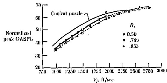
(a) Peak OASPL.
