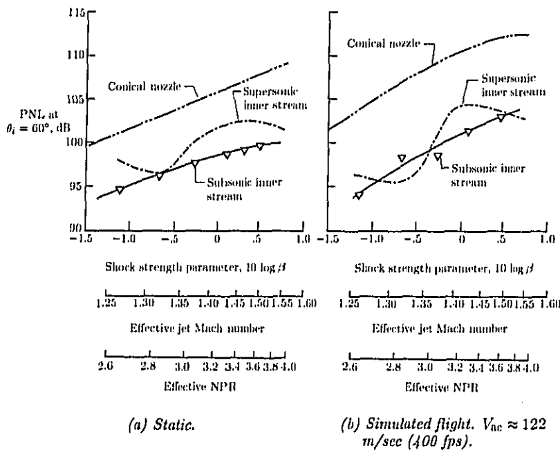
Figure 49. Effectiveness of subsonic inner stream operation on shock noise of coannular extended plug nozzle. Data scaled to A_T = 0.903 \text{ m}^2 ( 1400 \text{ in}^2 ) and 792-m (2400-ft) sideline. (Based on ref. 36.)
