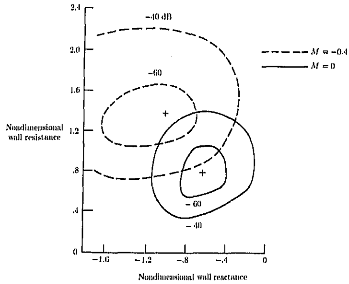
Figure 3. Contours of constant attenuation in length of \theta duct radii for circular duct. L/D = 3; \eta = \pi .
