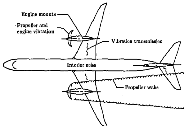
Figure 97. Sources and paths of structure-borne sound in twin-engine, propeller-driven airplane.
