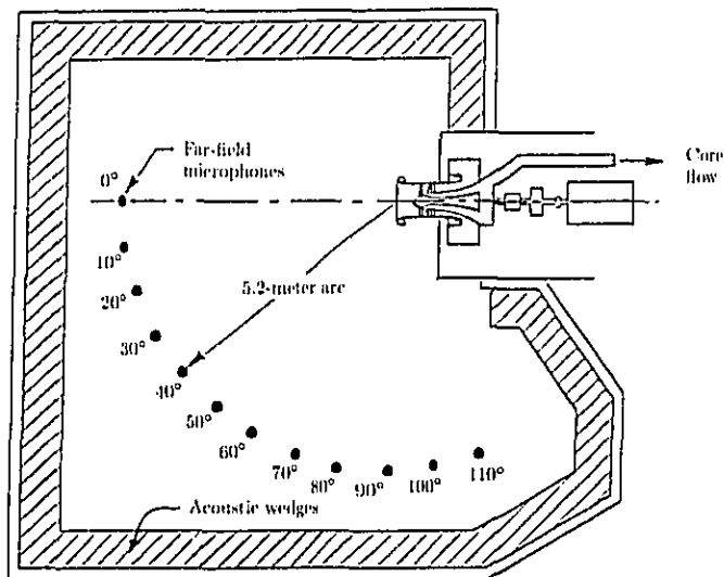
Figure 19. Typical scale model mounted in anechoic facility for development of treatment designs for inlet duct configuration.
