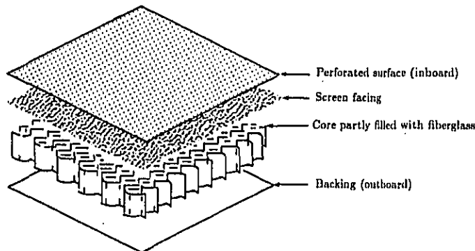
Figure 59. Components of sound-absorbing panel for airplane interior. (From ref. 135.)
