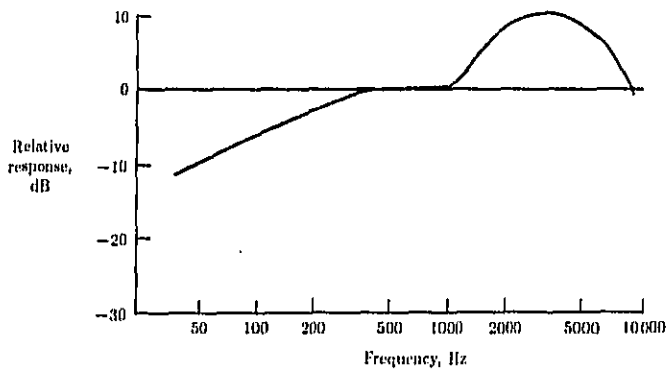
Figure 7. Relative response of the D-weighting filter.
