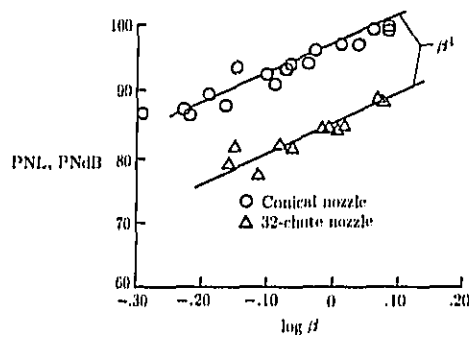
(a) PNL at \theta_i = 50^\circ .
