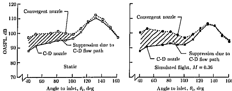
(c) OASPL directivity of convergent and C-D nozzles at C-D nozzle design conditions.
