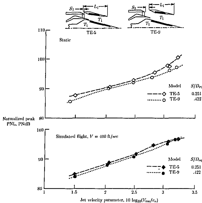
Figure 32. Influence of ejector spacing on normalized peak PNL of 20-shallow-chute suppressor nozzle (dual flow). 2400-ft sideline; A_T = 1400 \text{ in}^2 ; standard day (59° F, 70 percent relative humidity). (Based on ref. 25.)
