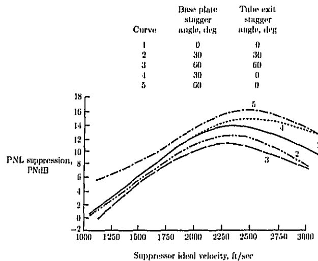
(a) Acoustic performance; 1500-ft sideline; A_T/A_j = 2.27 .
