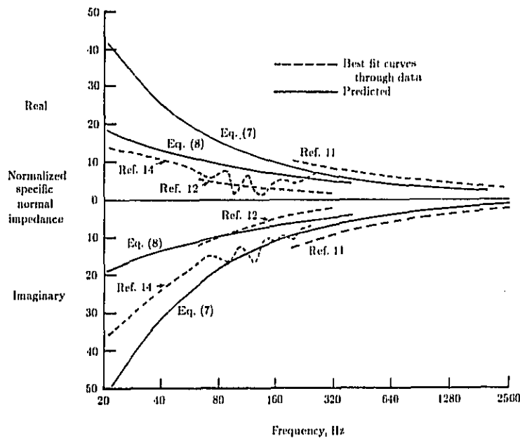
Figure 5. Normalized resistive (real) and reactive (imaginary) components of specific normal impedance for grass-covered grounds as a function of frequency. \sigma_e = 150 \times 10^3 Pa-sec/m 2 assumed in equations (7) and (8).
